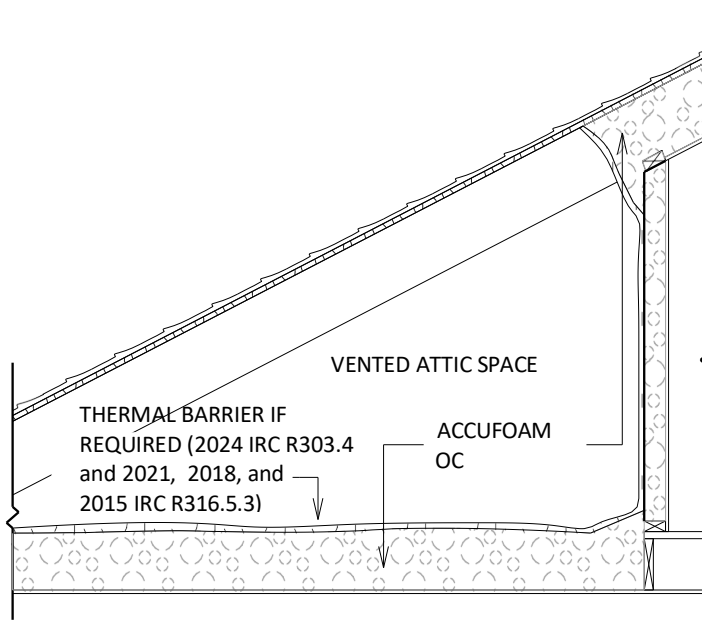
ATTIC KNEE WALL OPEN CELL
