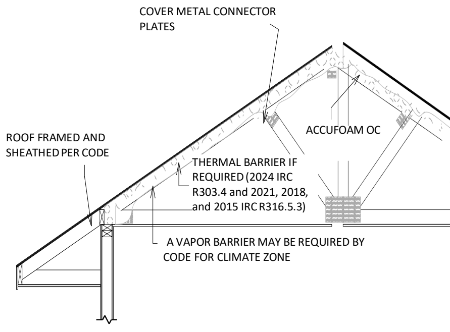
UNVENTED ATTIC INSULATED ROOF DECK OPEN CELL
